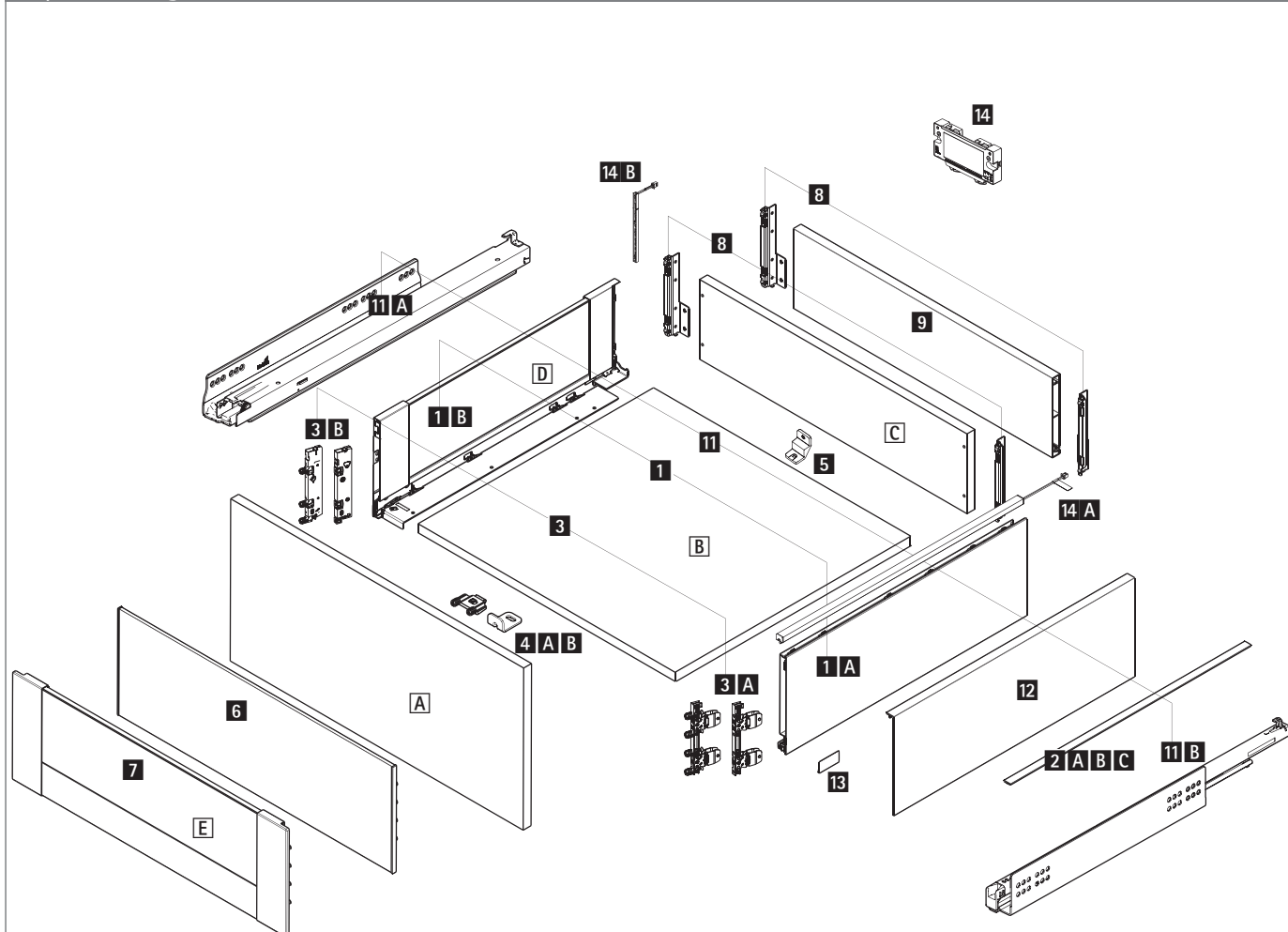
Exploded diagram
